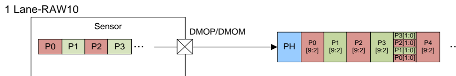
1 Lane Output Format
