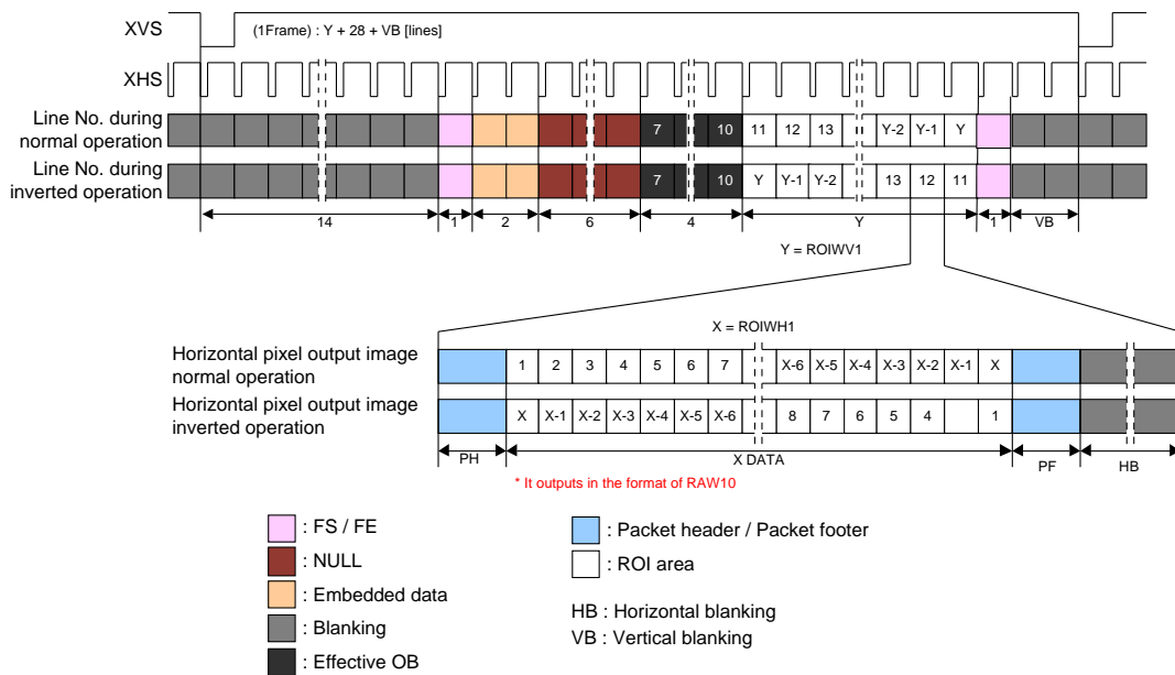
Drive Timing Chart for Serial Output in ROI Mode
