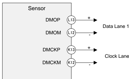
Relationship between Pin Name and MIPI Output Lane
