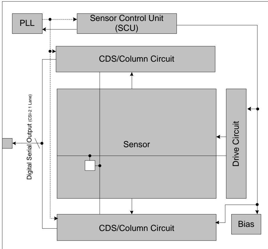
Block Diagram
